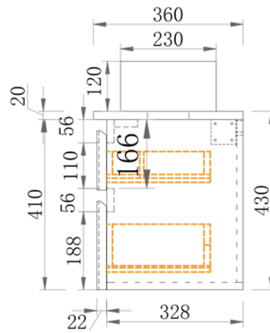
Section Side
