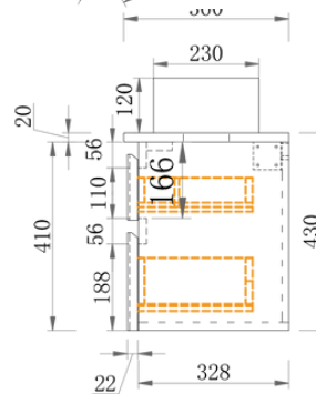
Section Side
